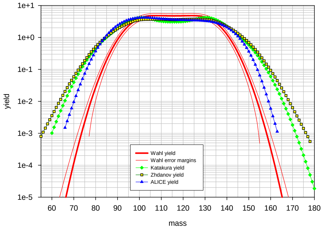
Benchmark B: ^{241}\text{Am} at 100 MeV, post neutron emission mass distribution
